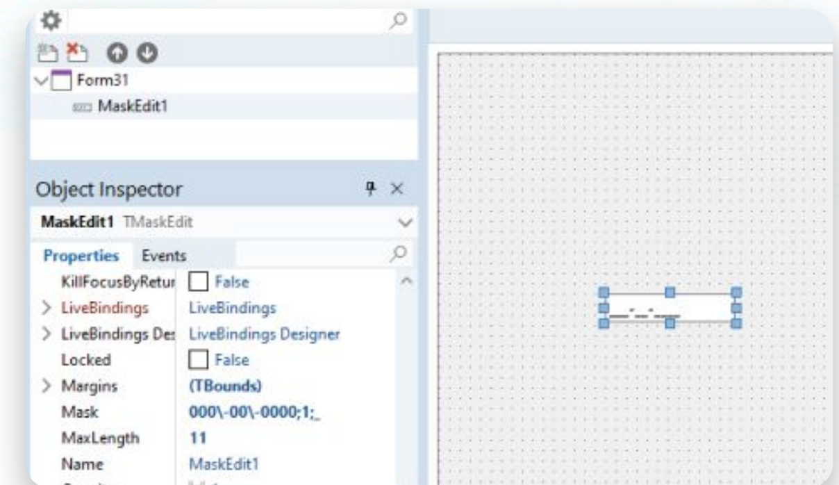
MaskEdit control
